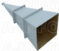
LB-187-25-A Standard Gain Horn Antenna 3.95-5.85GHz 25dB Gain Rectangular Waveguide Interface
